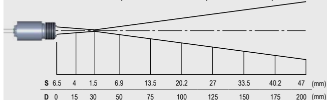
CSmicro 3ML CF1 optics, D:S = 22:1 (far field 3,5:1)
