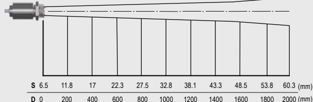
CSmicro 3MH SF optics, D:S = 33:1
