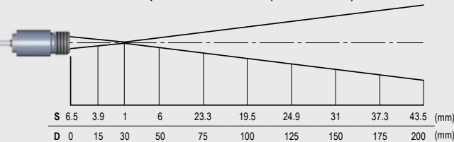
CSmicro 3MH CF1 optics, D:S = 33:1 (far field 4:1)
