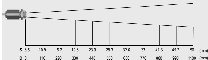
CSmicro 3ML SF optics, D:S = 22:1
