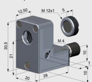
Air purge with integrated CF optics (ACCTAPLCF)
