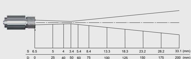
CF optics D:S = 15:1 (far field = 5:1)
