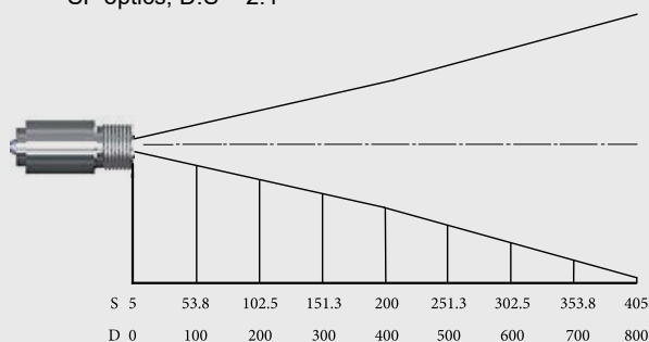
SF optics, D:S = 2:1
