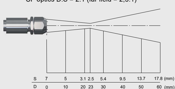
CF optics D:S = 2:1 (far field = 2,5:1)
