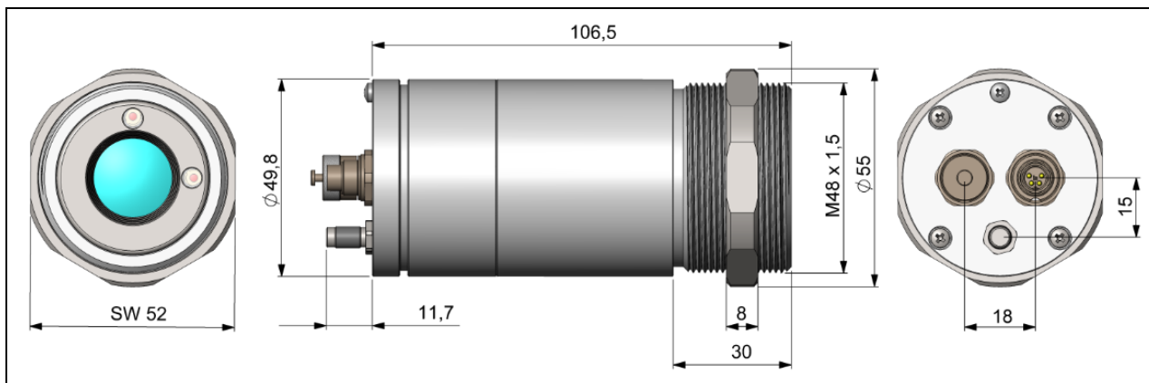
CSvideo sensing head
