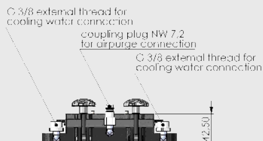
Laminar AirPurge: Connections
