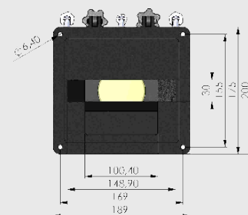
Laminar AirPurge: Line scan model
