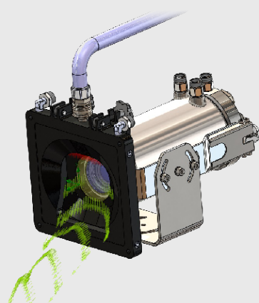
Orthogonal airflow
